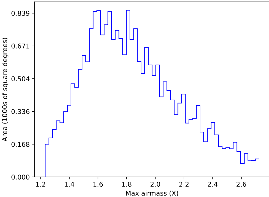
no_high_blob_v3.3_10yrs All sky u band: Max airmass
