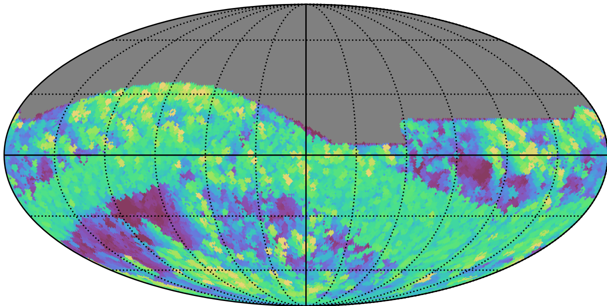
no_high_blob_v3.3_10yrs All sky r band: Max airmass
