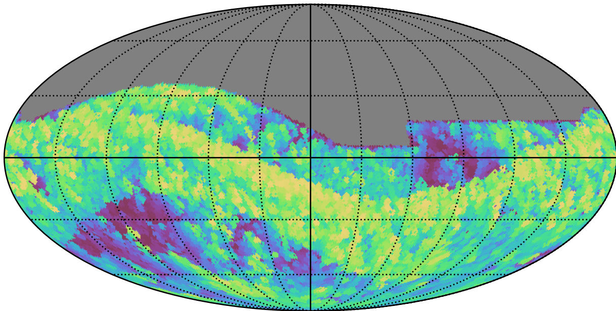
no_high_blob_v3.3_10yrs All sky i band: Max airmass
