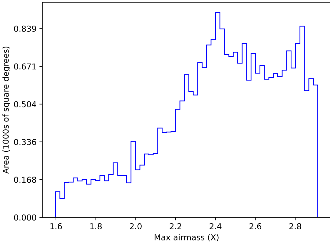
no_high_blob_v3.3_10yrs All sky i band: Max airmass
