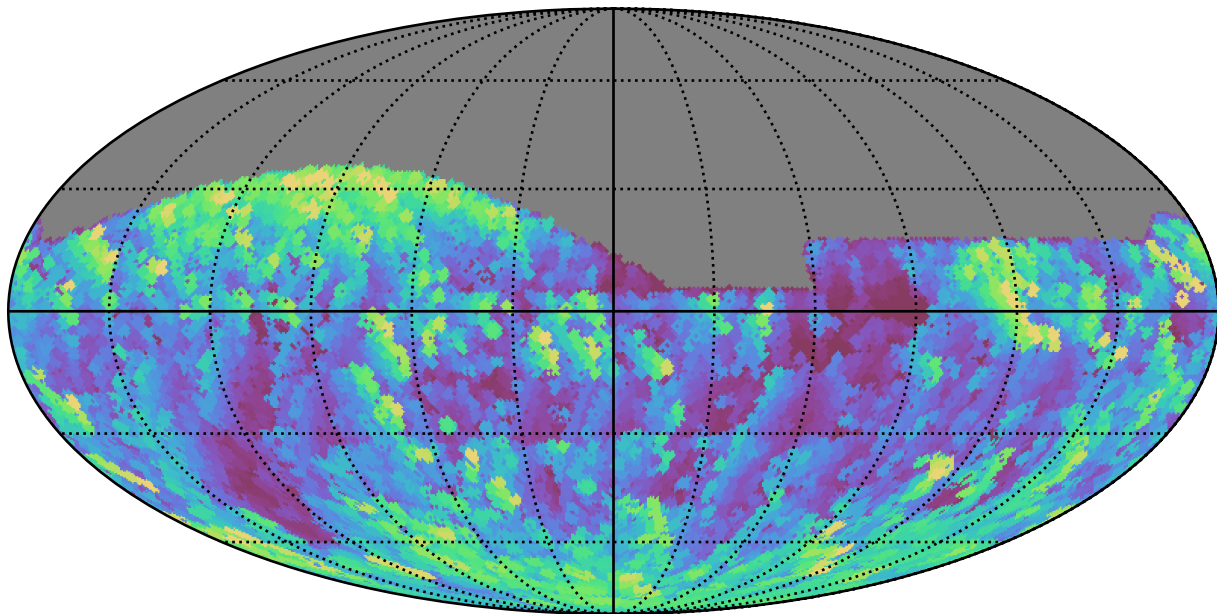
no_high_blob_v3.3_10yrs All sky g band: Max airmass
