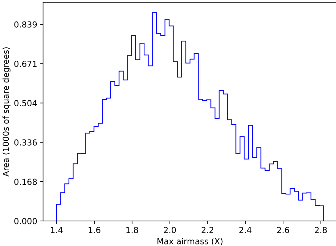
no_high_blob_v3.3_10yrs All sky g band: Max airmass
