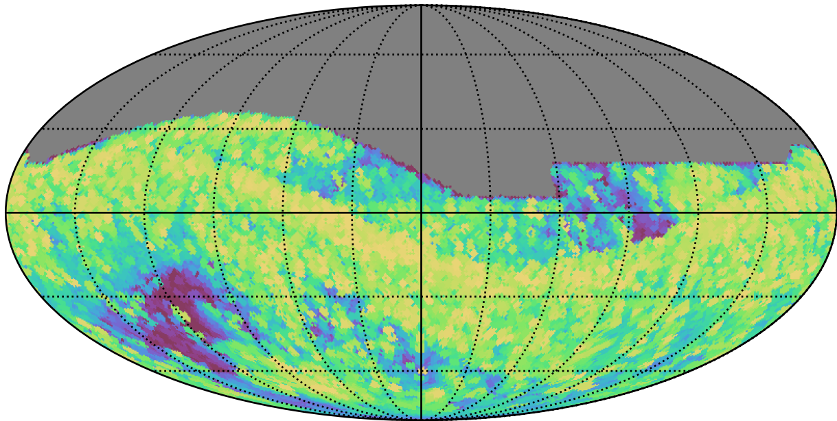
no_high_blob_v3.3_10yrs All sky all bands: Max airmass
