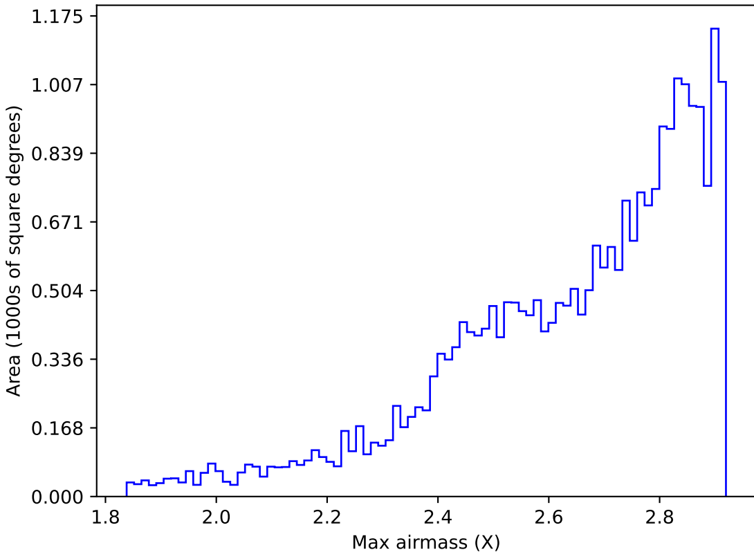
no_high_blob_v3.3_10yrs All sky all bands: Max airmass
