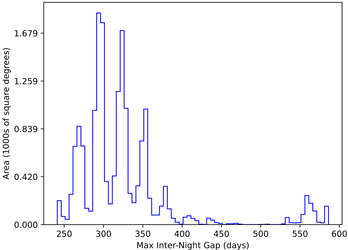
no_high_blob_v3.3_10yrs WFD y band: Max Inter-Night Gap
