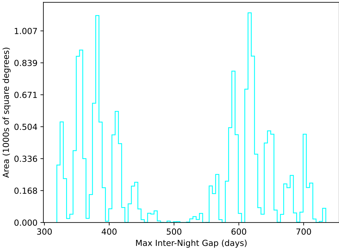
no_high_blob_v3.3_10yrs WFD u band: Max Inter-Night Gap
