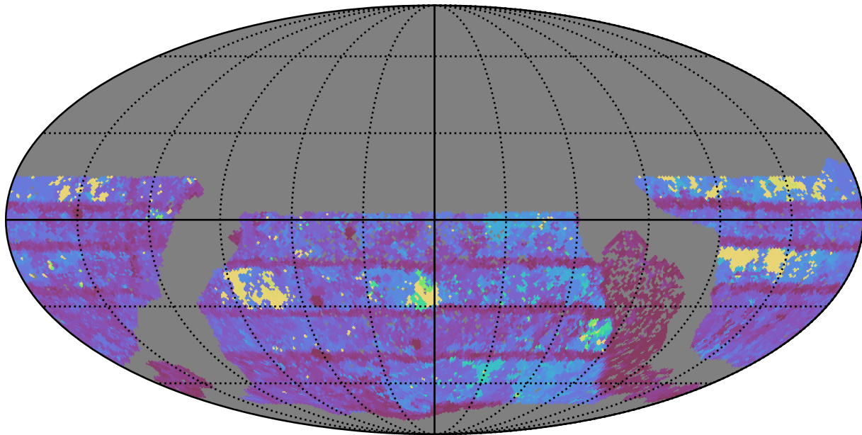
no_high_blob_v3.3_10yrs WFD r band: Max Inter-Night Gap
