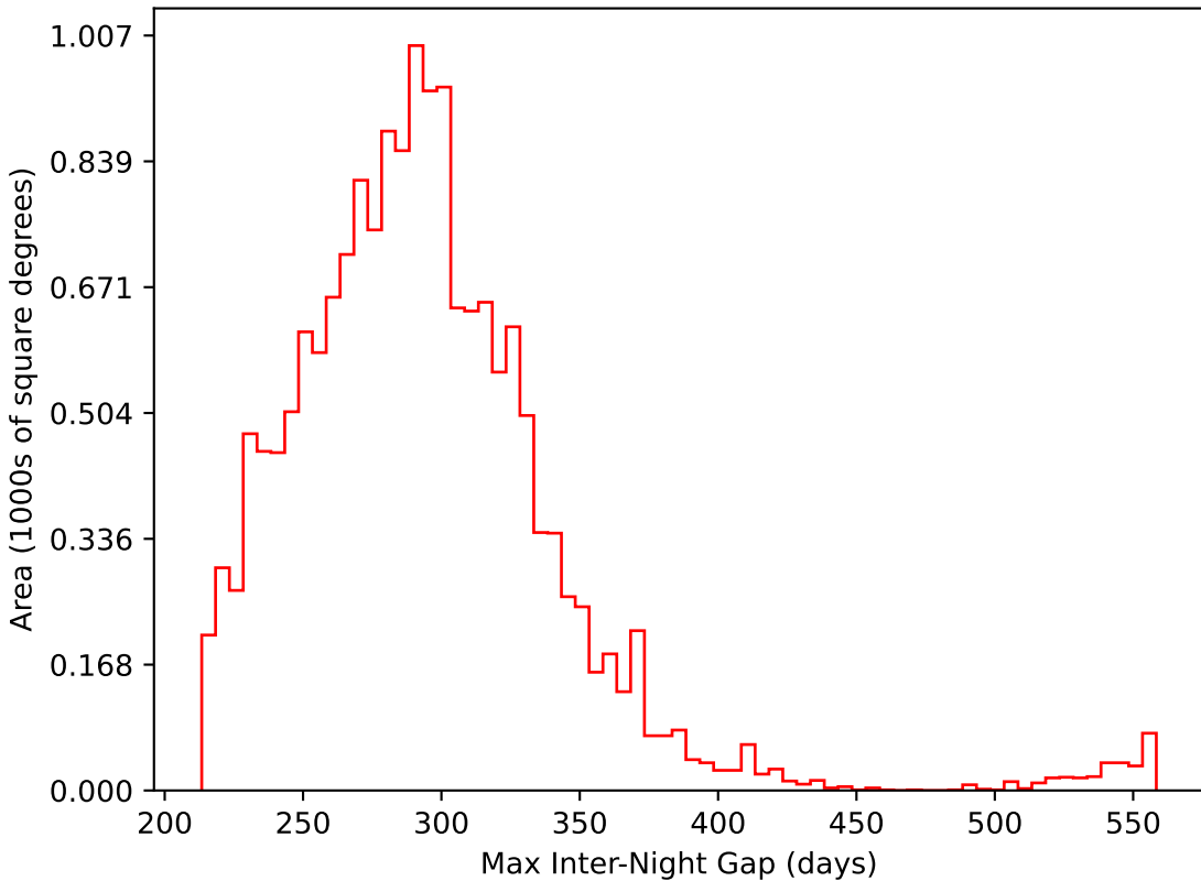
no_high_blob_v3.3_10yrs WFD i band: Max Inter-Night Gap
