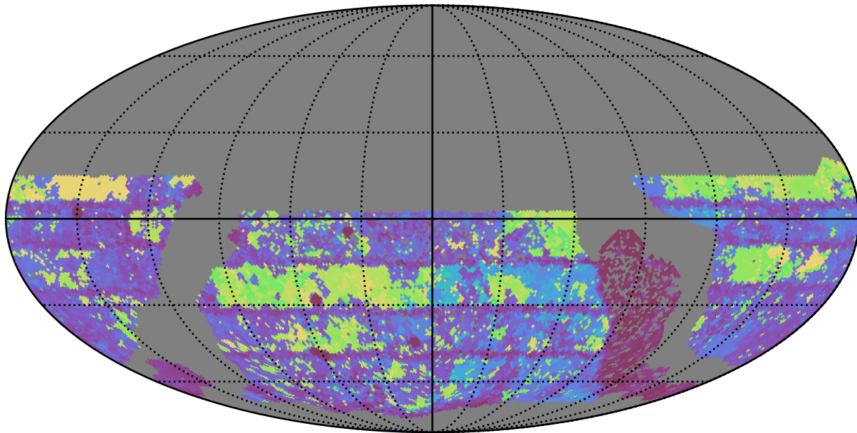
no_high_blob_v3.3_10yrs WFD g band: Max Inter-Night Gap
