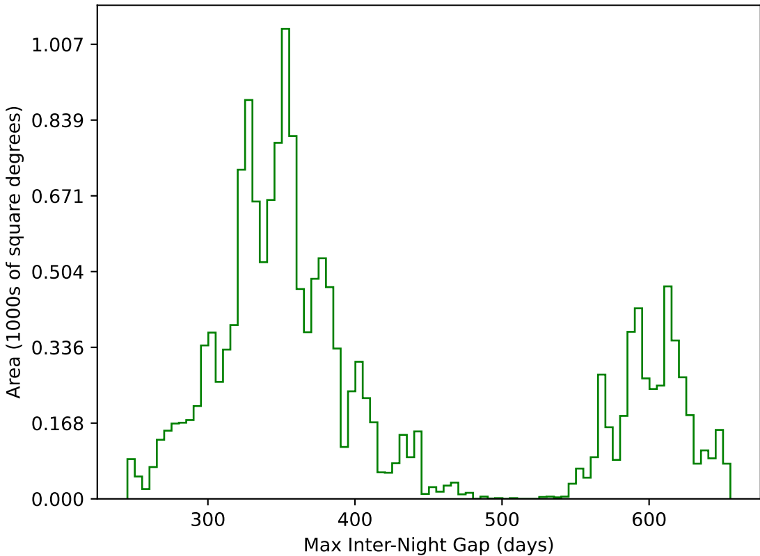
no_high_blob_v3.3_10yrs WFD g band: Max Inter-Night Gap
