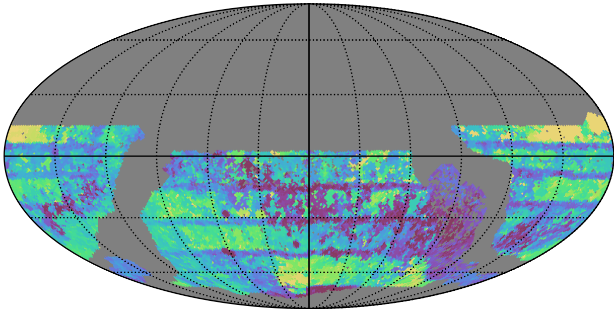
no_high_blob_v3.3_10yrs WFD all bands: Max Inter-Night Gap
