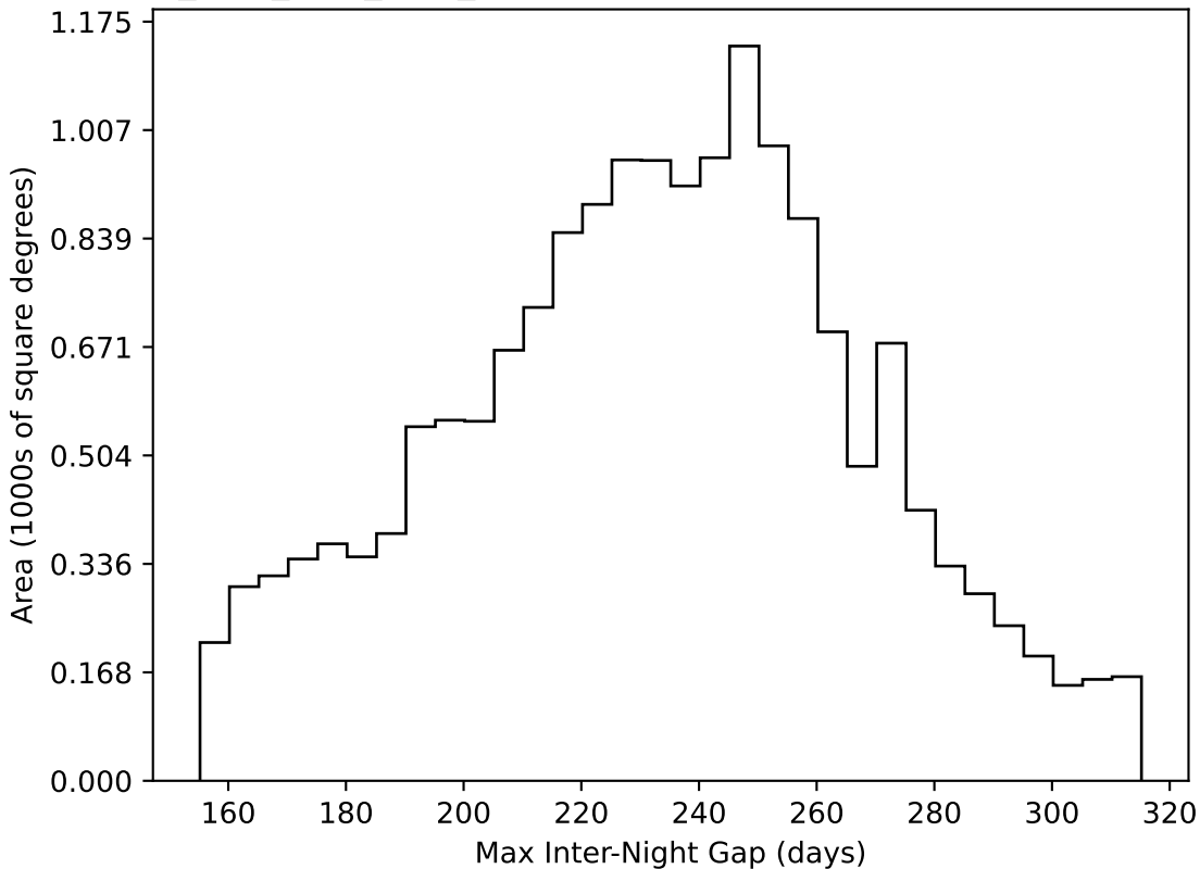
no_high_blob_v3.3_10yrs WFD all bands: Max Inter-Night Gap
