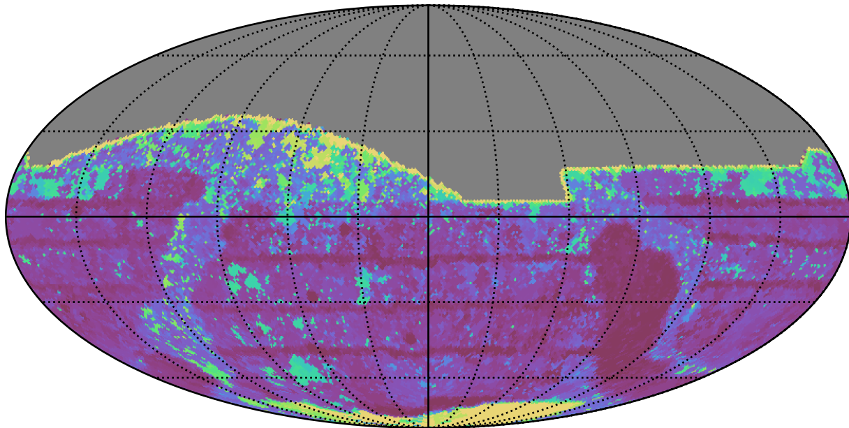
no_high_blob_v3.3_10yrs All sky z band: Max Inter-Night Gap
