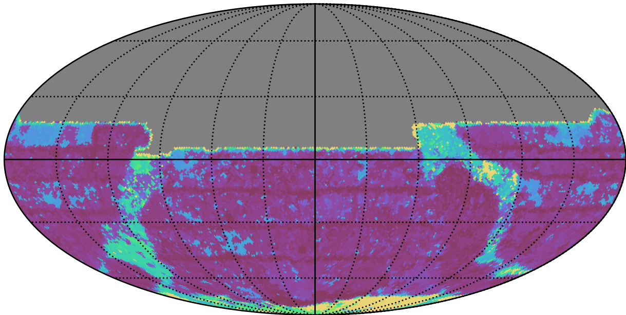
no_high_blob_v3.3_10yrs All sky y band: Max Inter-Night Gap
