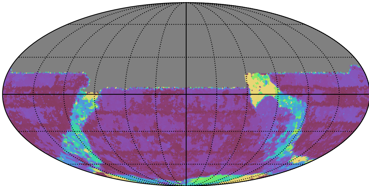
no_high_blob_v3.3_10yrs All sky u band: Max Inter-Night Gap
