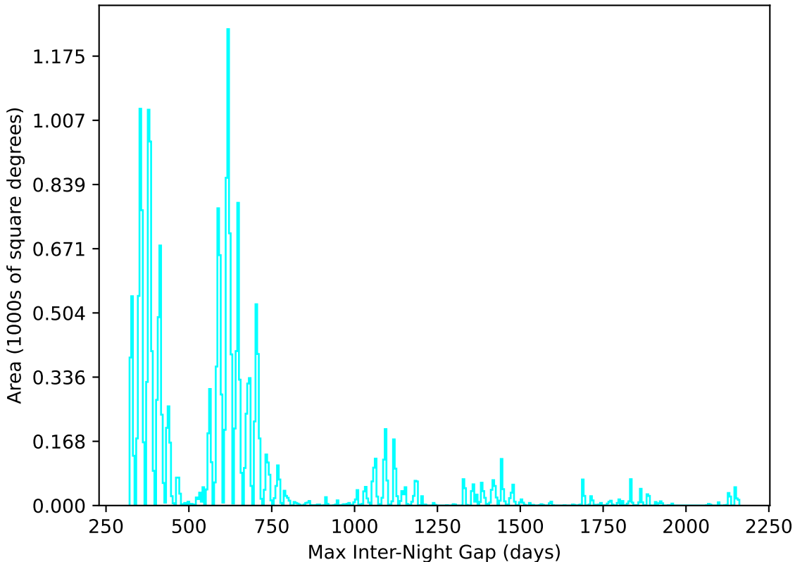
no_high_blob_v3.3_10yrs All sky u band: Max Inter-Night Gap
