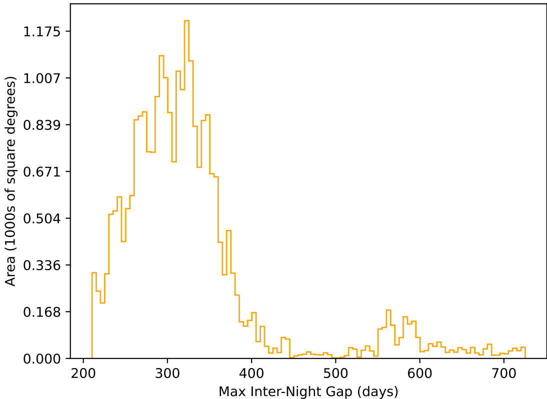
no_high_blob_v3.3_10yrs All sky r band: Max Inter-Night Gap
