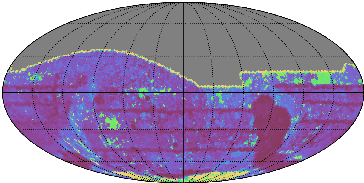
no_high_blob_v3.3_10yrs All sky i band: Max Inter-Night Gap
