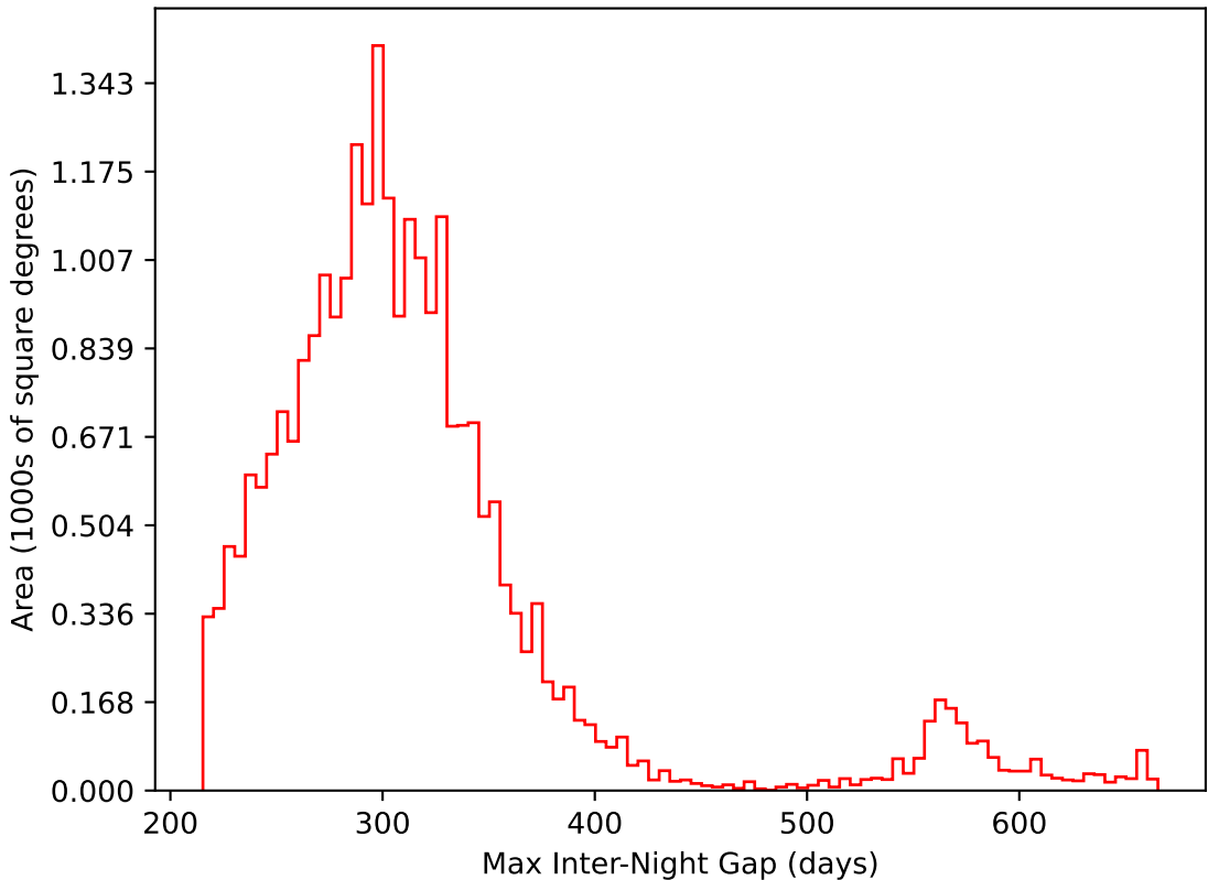
no_high_blob_v3.3_10yrs All sky i band: Max Inter-Night Gap
