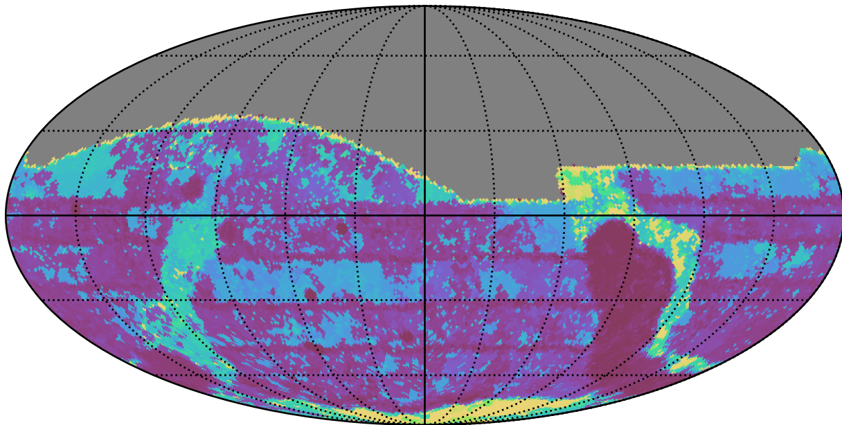
no_high_blob_v3.3_10yrs All sky g band: Max Inter-Night Gap
