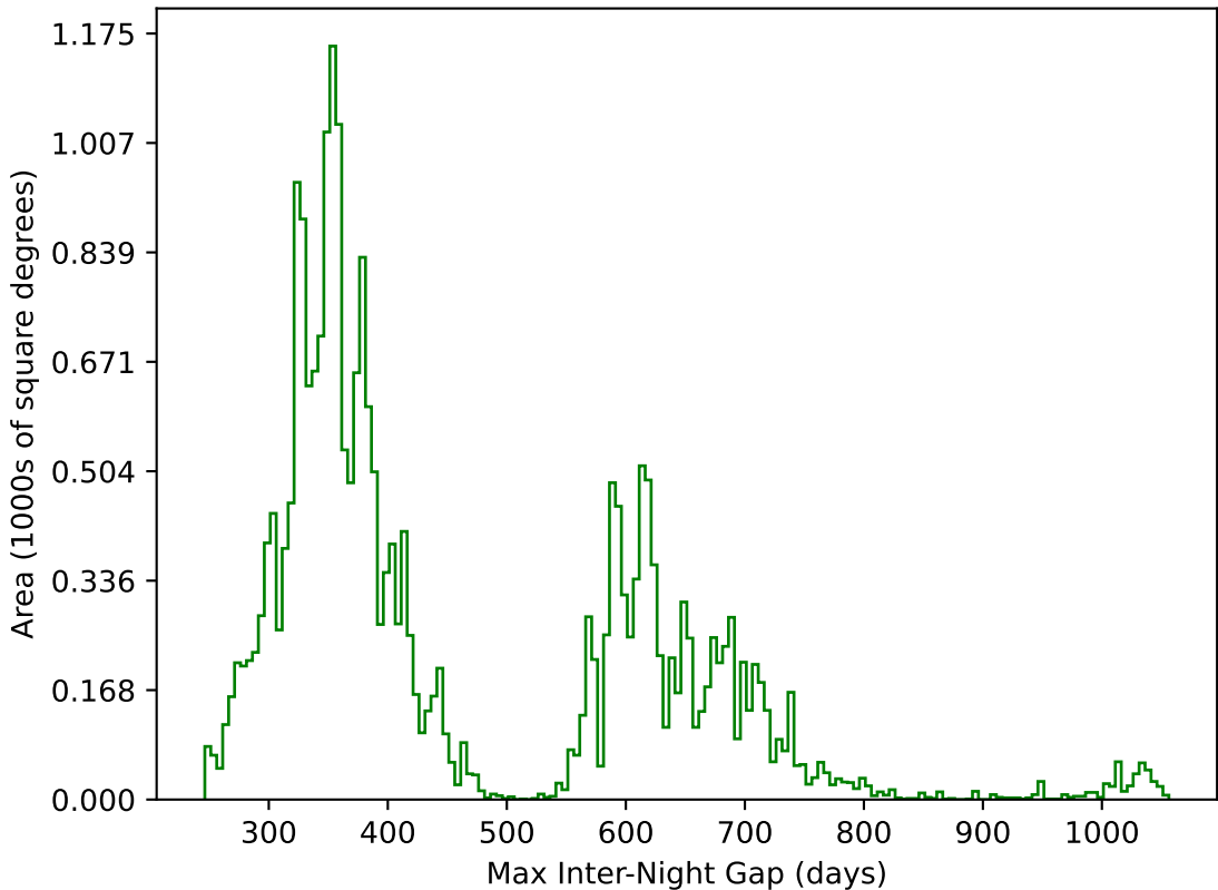
no_high_blob_v3.3_10yrs All sky g band: Max Inter-Night Gap
