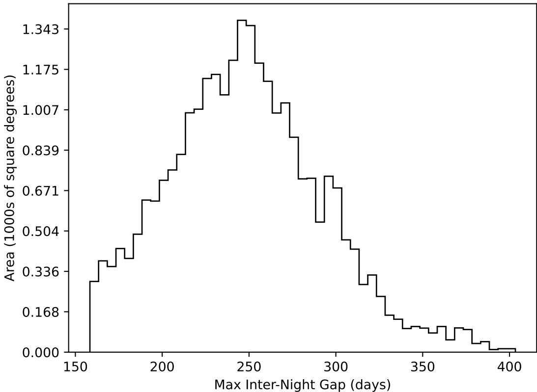
no_high_blob_v3.3_10yrs All sky all bands: Max Inter-Night Gap
