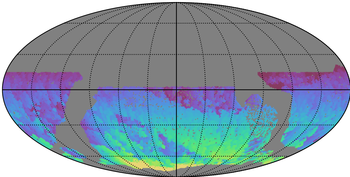
no_high_blob_v3.3_10yrs WFD z band: Max HA
