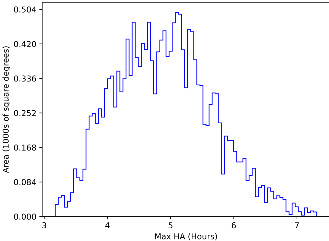
no_high_blob_v3.3_10yrs WFD z band: Max HA
