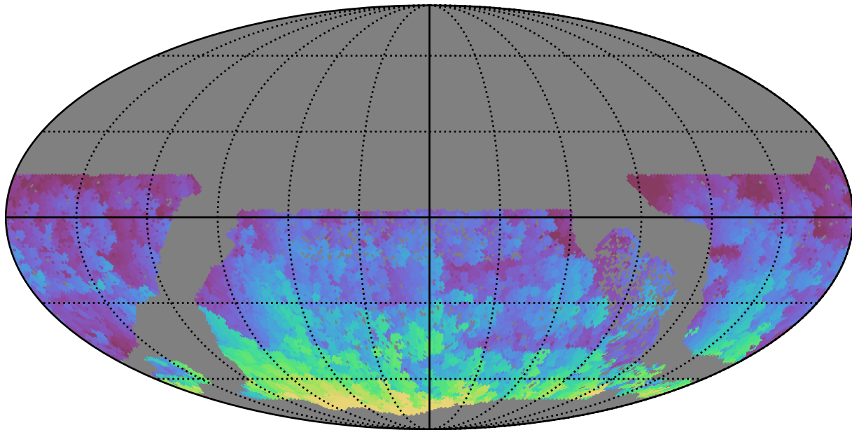
no_high_blob_v3.3_10yrs WFD r band: Max HA
