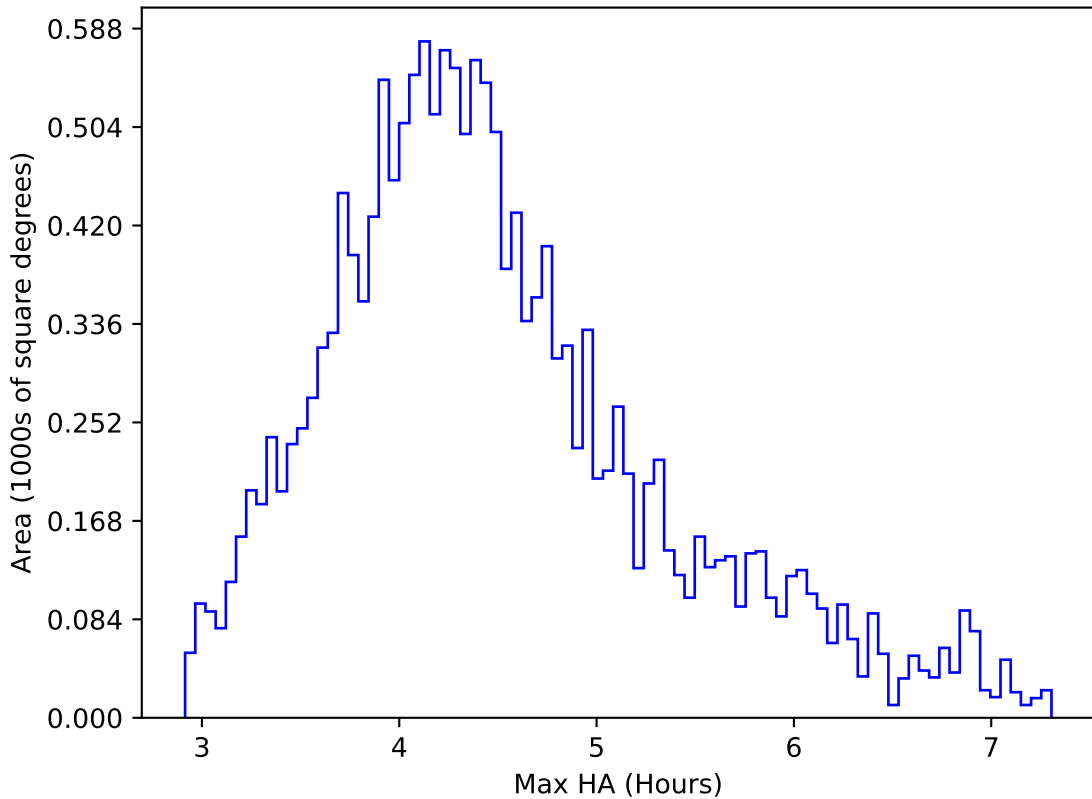
no_high_blob_v3.3_10yrs WFD r band: Max HA
