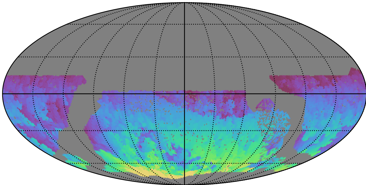
no_high_blob_v3.3_10yrs WFD i band: Max HA
