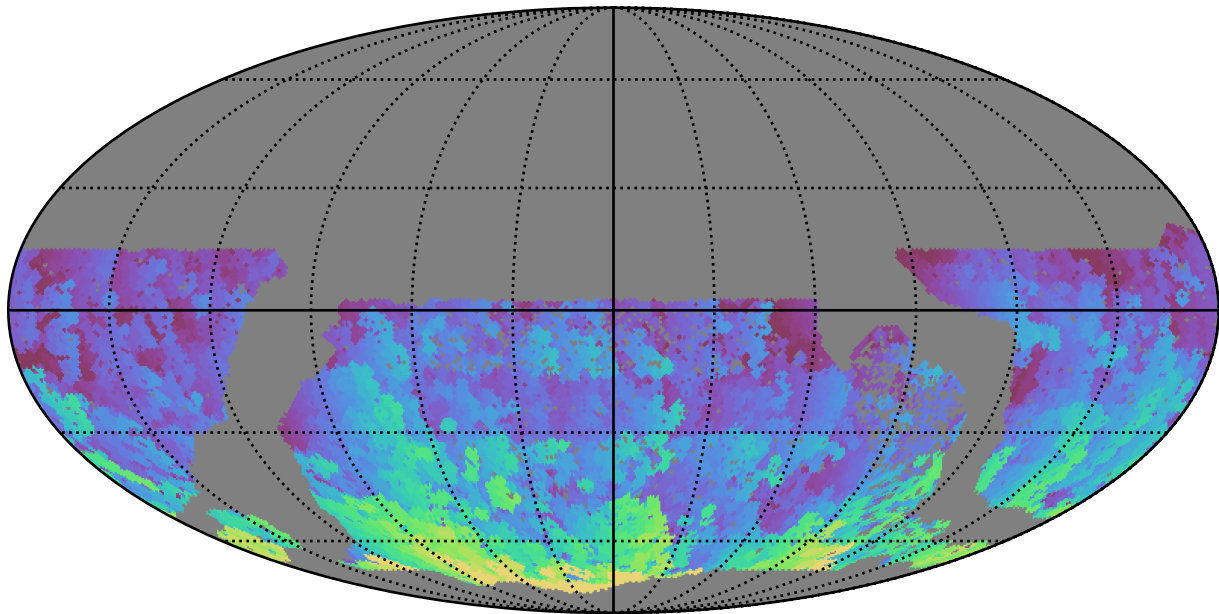
no_high_blob_v3.3_10yrs WFD g band: Max HA
