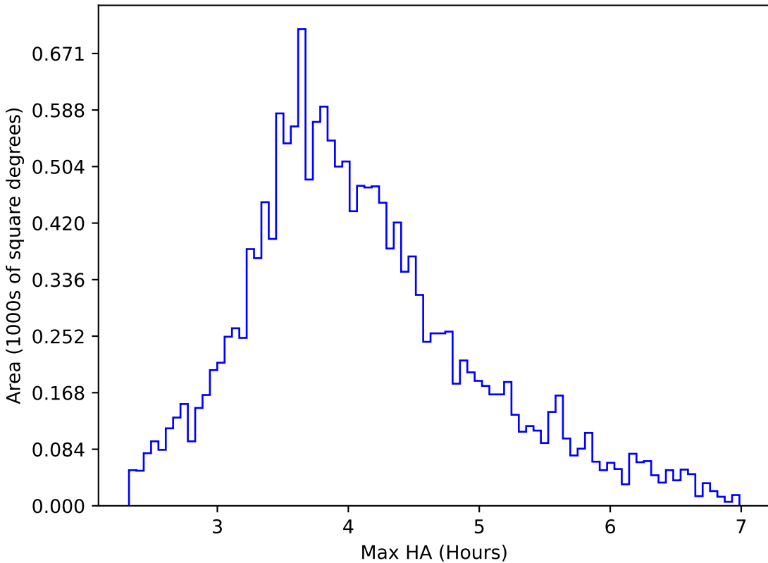
no_high_blob_v3.3_10yrs WFD g band: Max HA
