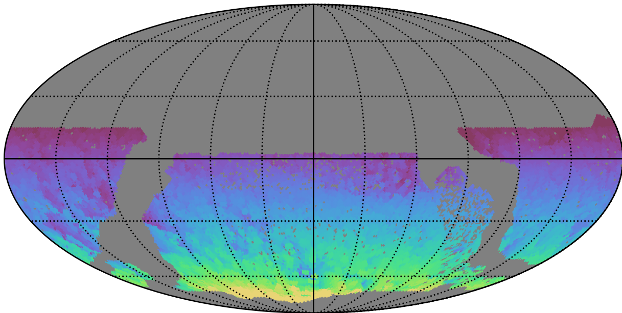
no_high_blob_v3.3_10yrs WFD all bands: Max HA
