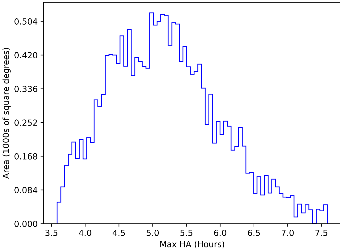
no_high_blob_v3.3_10yrs WFD all bands: Max HA
