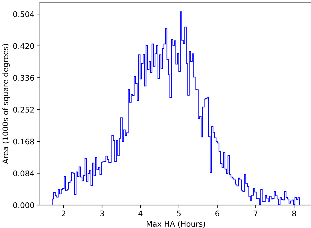
no_high_blob_v3.3_10yrs All sky z band: Max HA
