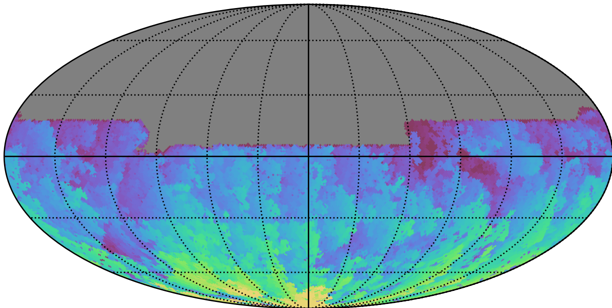
no_high_blob_v3.3_10yrs All sky u band: Max HA
