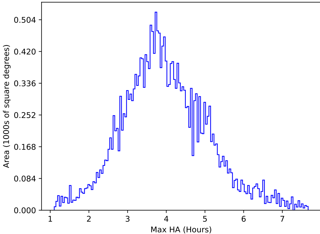
no_high_blob_v3.3_10yrs All sky u band: Max HA
