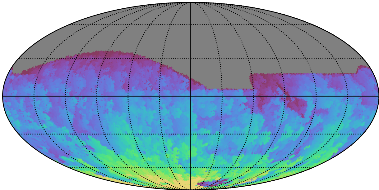
no_high_blob_v3.3_10yrs All sky r band: Max HA
