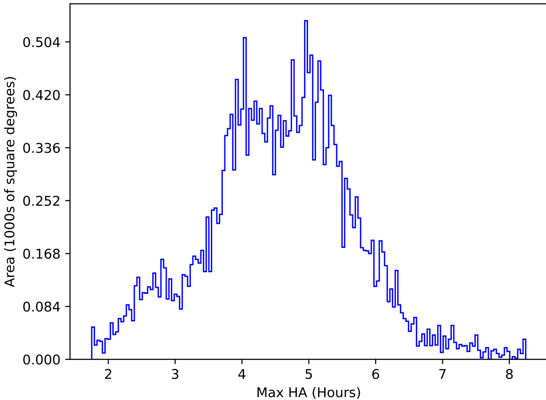
no_high_blob_v3.3_10yrs All sky i band: Max HA
