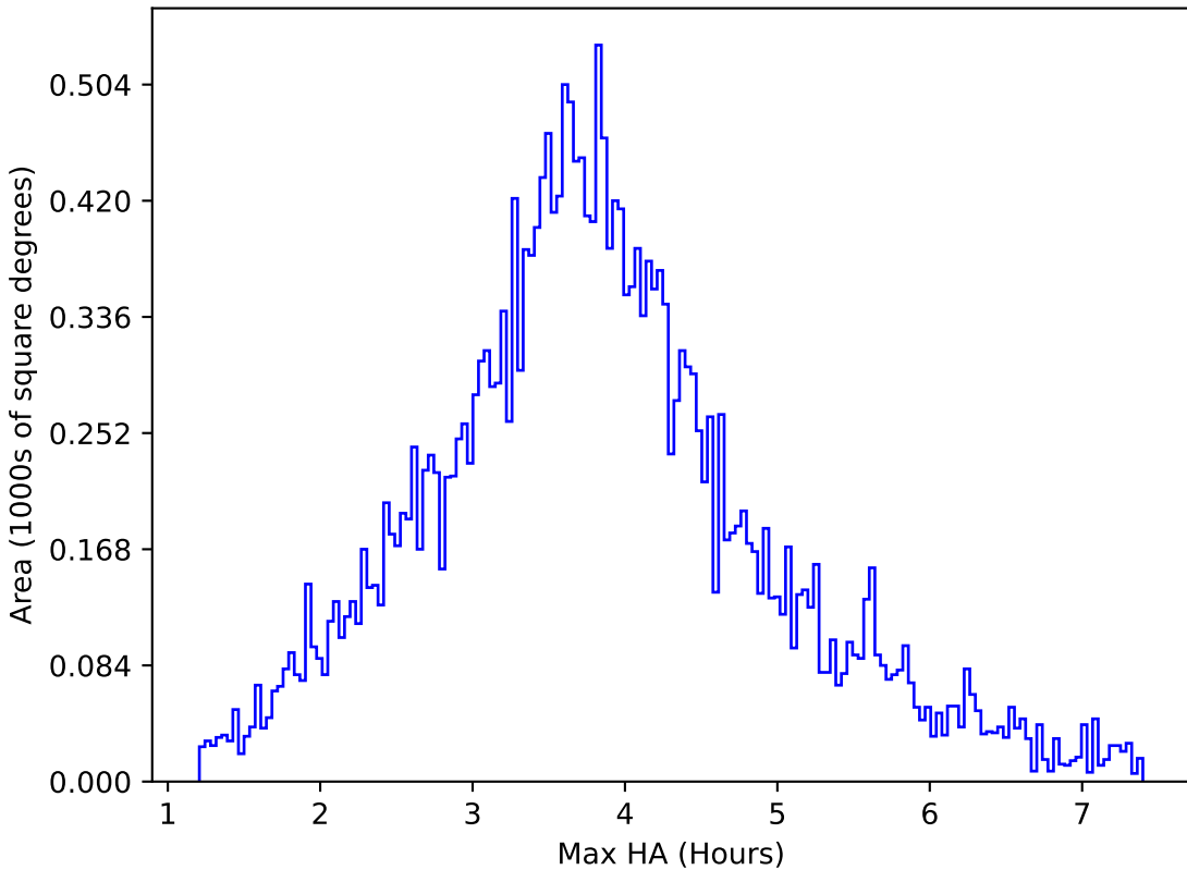
no_high_blob_v3.3_10yrs All sky g band: Max HA
