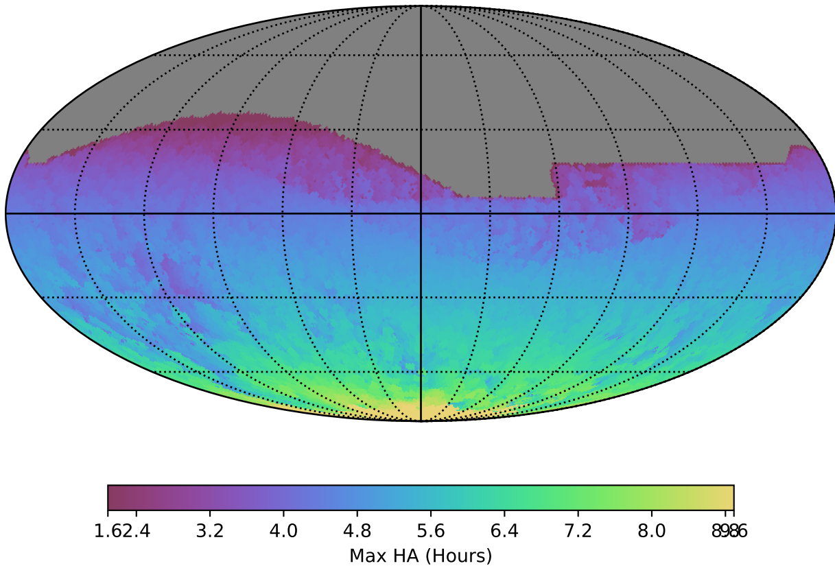
no_high_blob_v3.3_10yrs All sky all bands: Max HA
