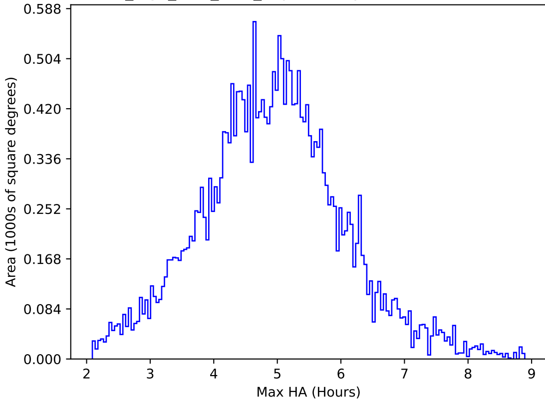
no_high_blob_v3.3_10yrs All sky all bands: Max HA
