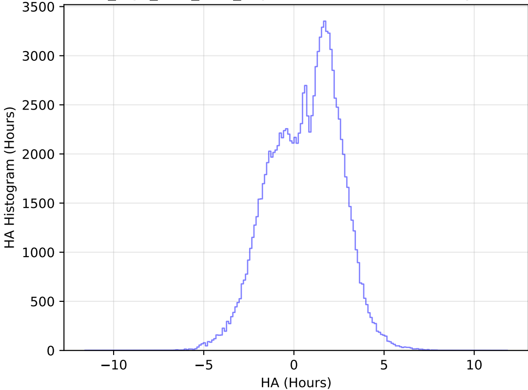
no_high_blob_v3.3_10yrs WFD u band: HA Histogram
