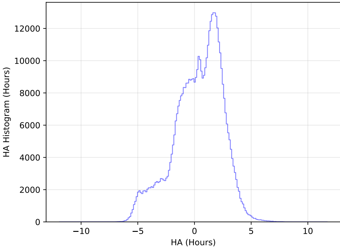
no_high_blob_v3.3_10yrs WFD r band: HA Histogram
