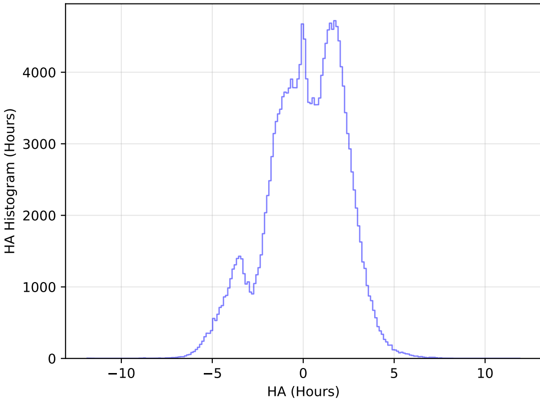
no_high_blob_v3.3_10yrs WFD g band: HA Histogram
