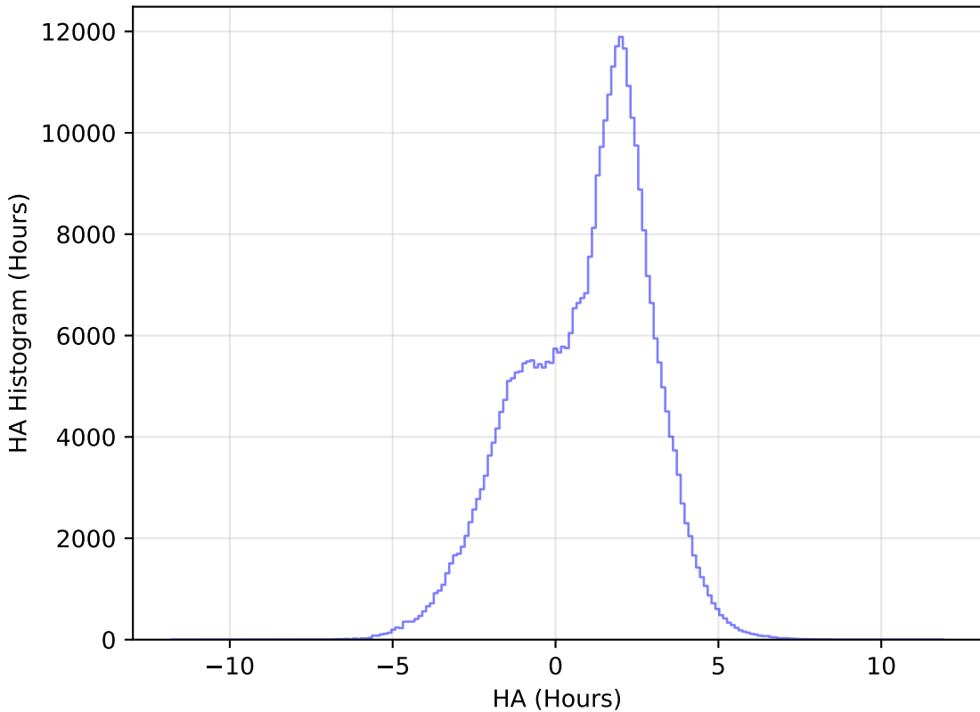
no_high_blob_v3.3_10yrs All sky y band: HA Histogram
