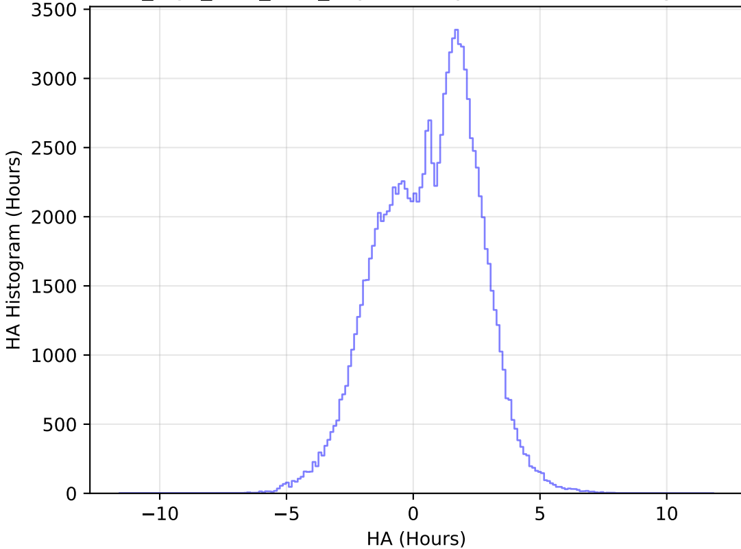
no_high_blob_v3.3_10yrs All sky u band: HA Histogram
