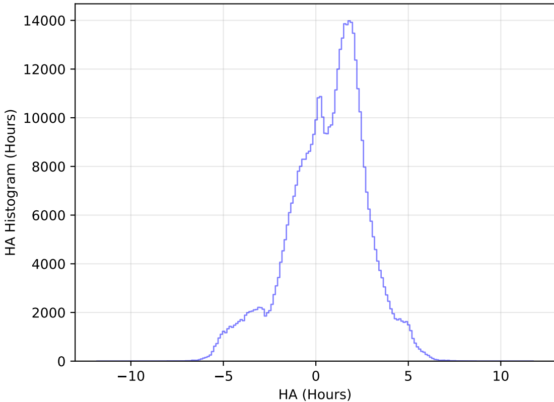
no_high_blob_v3.3_10yrs All sky i band: HA Histogram
