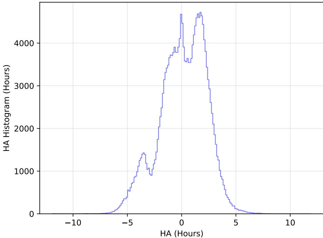
no_high_blob_v3.3_10yrs All sky g band: HA Histogram
